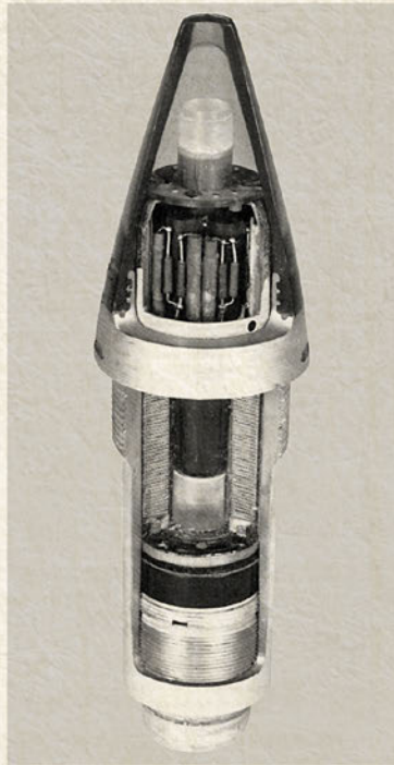
Figure 2. The VT fuze.
