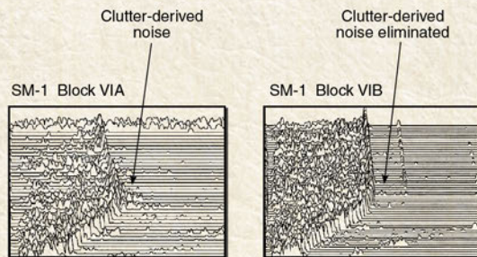
Figure 6. Clutter-derived noise comparison.
