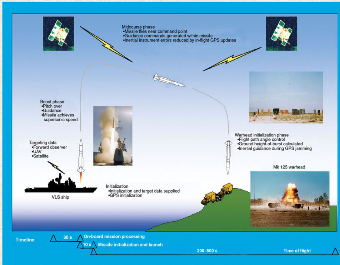
Figure 12. LASM concept of operations.
