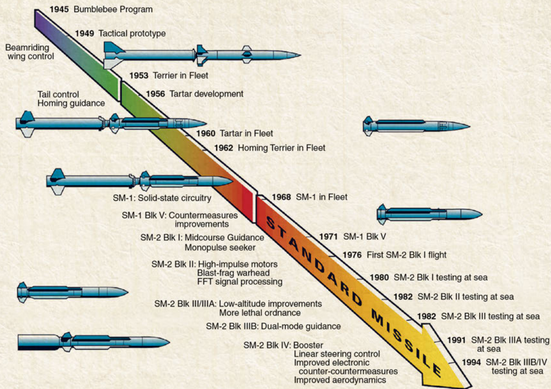
Figure 1. The evolution of in-service Standard Missiles.
