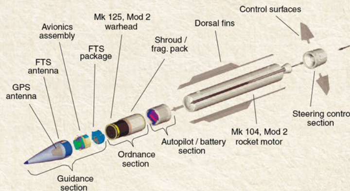
Figure 11. Land Attack Standard Missile (SM-4).
