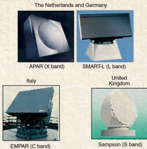
Figure 16. SM Allied navy multifunction radar options.
