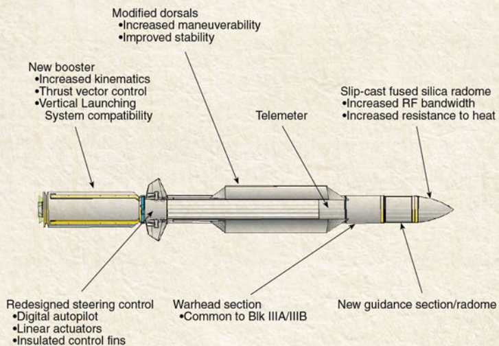
Figure 7. SM-2 Block IV.
