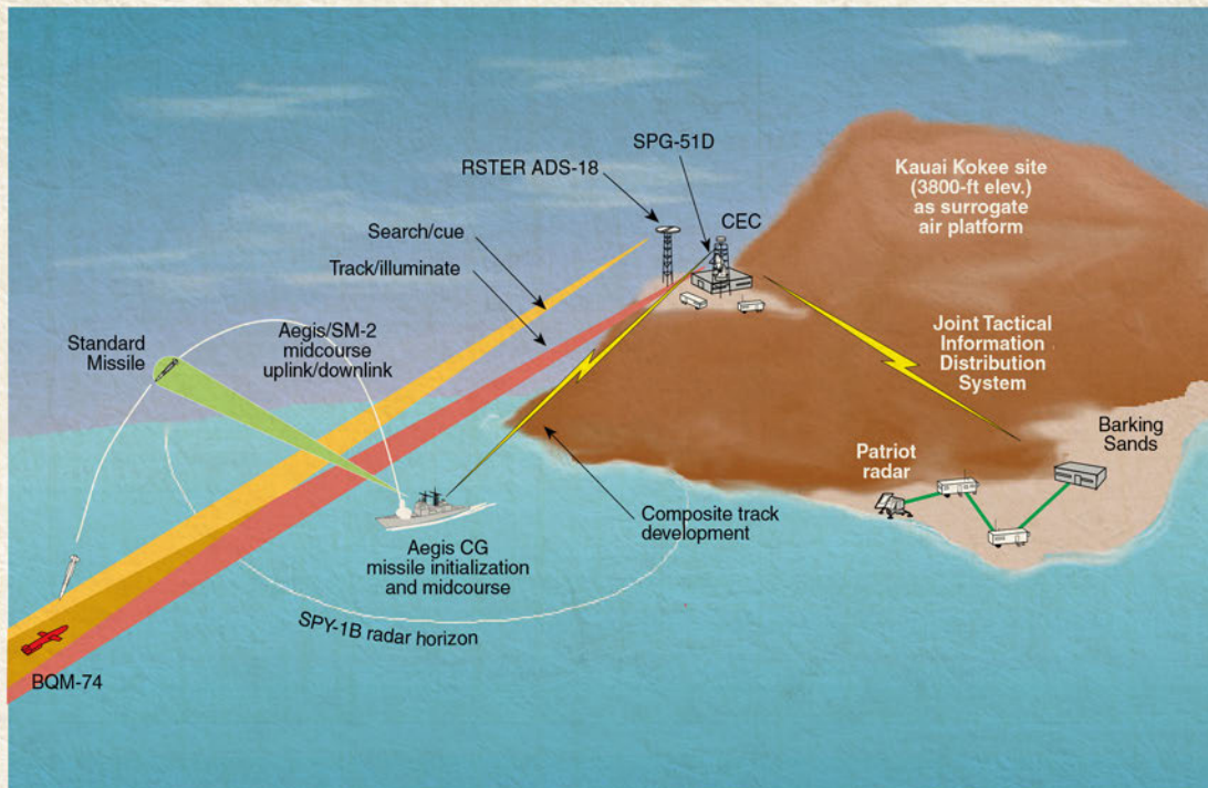
Figure 14. Mountain Top engagement architecture.
