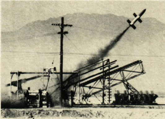
Figure 2 — Early subsonic test vehicle used in the development of TALOS guidance and control systems. This solid fuel rocket, developed in 1949, is shown being launched at Inyokern, Calif.
