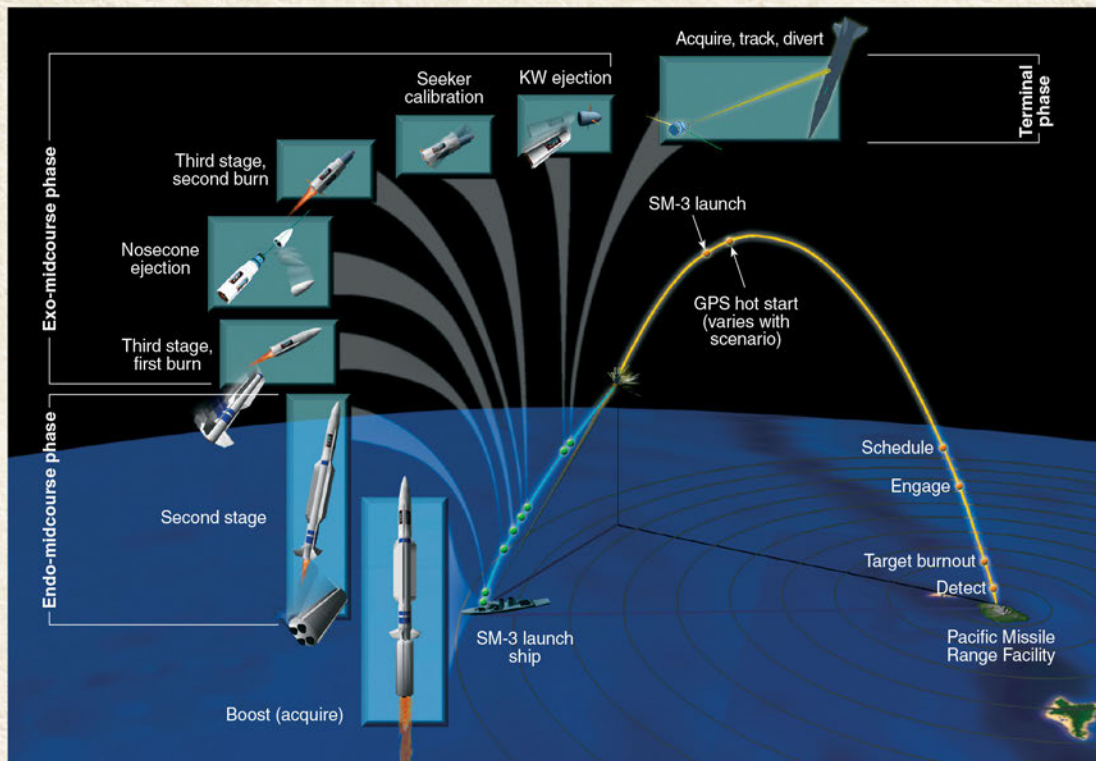
Figure 9. SM-3 concept of operations.
