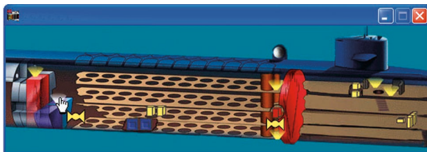
Figure 1. Navigator Window.
