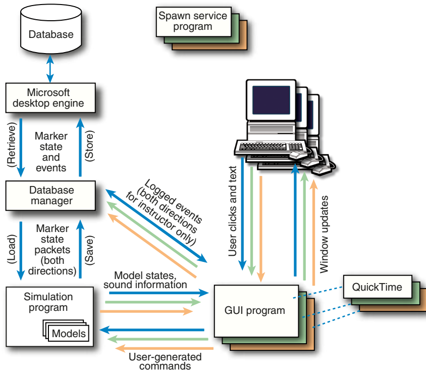
Figure 5. Simulation architecture.
