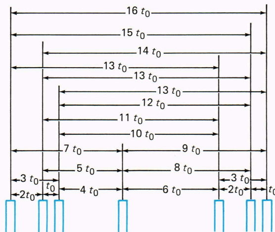
Figure 9 —Seven-pulse transmission sequence used for the determination of 17 lag autocorrelation functions of the backscattered signals. From the autocorrelation functions, one can derive the Doppler spectra by Fourier transformation.
