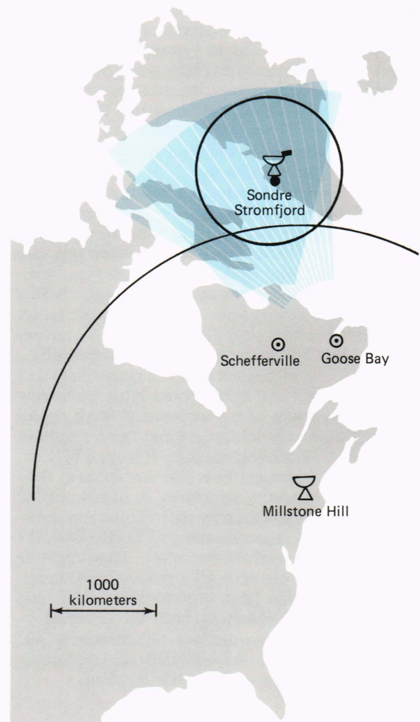
Figure 2 —Field of view of APL's HF radar at Goose Bay. The radar can be pointed electronically into any of 16 possible directions with a resolution cell defined by the small dark-shaded region along one of the beams. Also shown are the nominal fields of view of the Sondre Stromfjord and Millstone Hill incoherent scatter radars and the planned field of view (light-shaded) of a French HF radar that will be located at Schefferville, Quebec. The French radar will be quite similar to the Goose Bay radar; together, they will be used for two-component measurements of irregularity drift.
