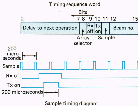
Figure 8 —Examples of timing sequencer control word and timing sequence. All time-critical radar functions are under the control of the timing sequencer. This device is a direct-memory-access-controlled buffer that receives 16 bit words from a software-generated timing sequence array within the computer memory. The bits of these control words determine the time delay to the next control word transfer, the antenna array selected, the status of the transmit/receive switch, the status of the transmit pulse, the status of the sample gate, and the antenna beam selected. Generally, the timing sequence is less than 500 words long.
