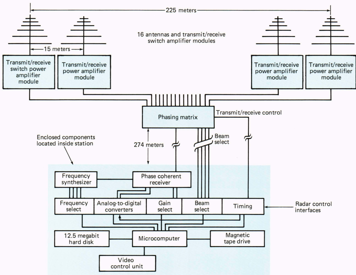
Figure 3 —Schematic diagram of the APL radar as it existed prior to the installation of the new receive-only array. Each antenna is driven by a 125-watt broadband solid-state power amplifier located at the base of its support tower. Each power amplifier module also contains transmit/receive (T/R) switches for routing the transmitted and received power. The power supplies for the modules are located in the shed containing the phasing matrix at the center of the antenna array, and the remainder of the equipment is located in the station 274 meters from the center of the array.
