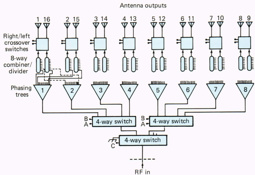
Figure 5 —Schematic diagram of the phasing matrix, which establishes a progressive time delay across the antenna array on transmission and reforms the beam on reception. The 4-way switches select one of eight possible branching networks (phasing trees). Each tree consists of power dividers and delay lines that produce a specific time delay across the 16 outputs and represents one possible beam direction. The crossover switches determine whether the selected beam points to the right or left of the array normal. On reception, the process is reversed, and the matrix reinforces only those signals from the preselected direction.
