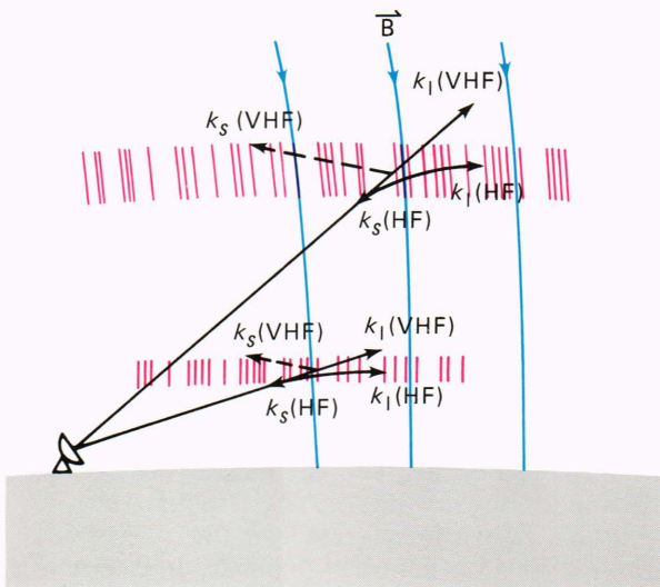
Figure 1 —Illustration of the manner in which VHF and higher frequency radar signals are scattered into space by very-high-latitude E- and F-region electron density irregularities. At HF frequencies, the radar signals are refracted toward the horizontal as they enter those two ionospheric layers. If the signals are propagating perpendicular to the magnetic field lines when they encounter a region of irregularities, the back-scattered signals will return to the radar.
